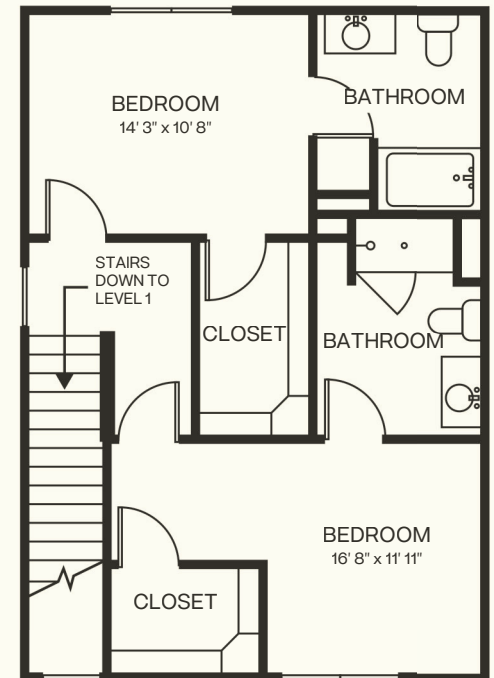
LEVEL 2
